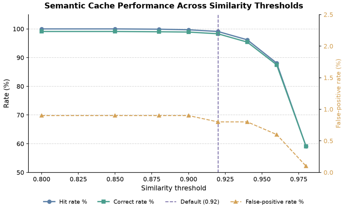
Figure 6.6: Cache hit rate and correctness rate as a function of the similarity threshold (left axis), with the false-positive rate on the magnified right axis. The system default of 0.92 is marked.
