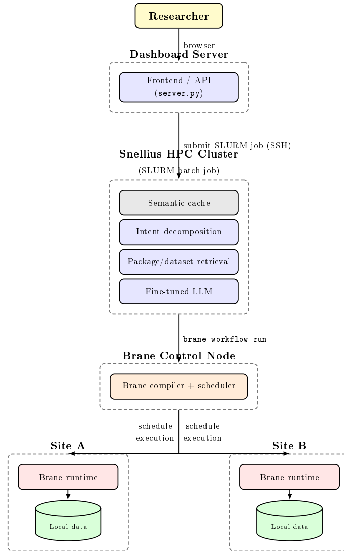
Figure 3.2: Physical deployment of the components shown in Figure 3.1
